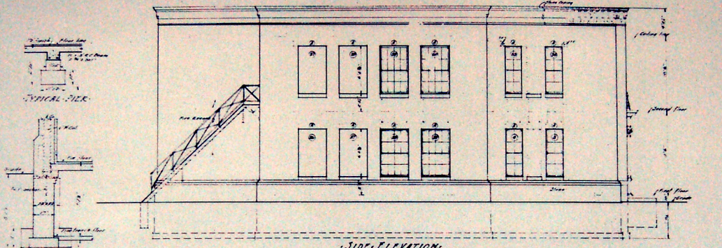
SIDE ELEVATION
