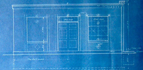
WEST ELEVATION SCALE 1/2" = 1'-0"
