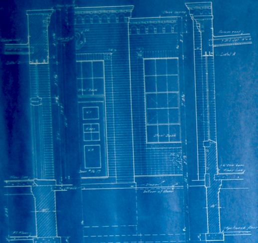
SECTION AT DOOR ELEVATION DETAIL AT ENTRANCE SCALE 1/2" = 1'-0"
