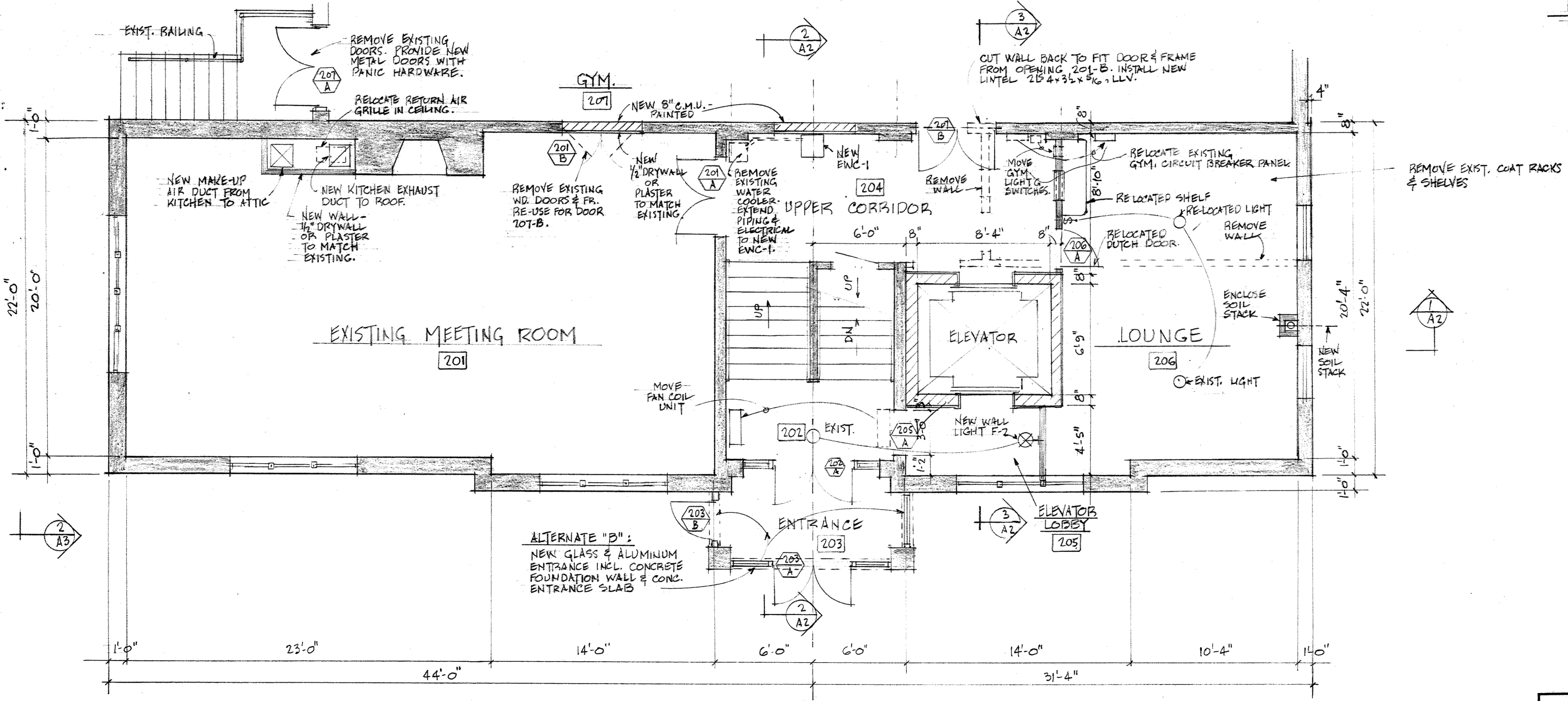
UPPER FLOOR PLAN 1/4" = 1'-0"
