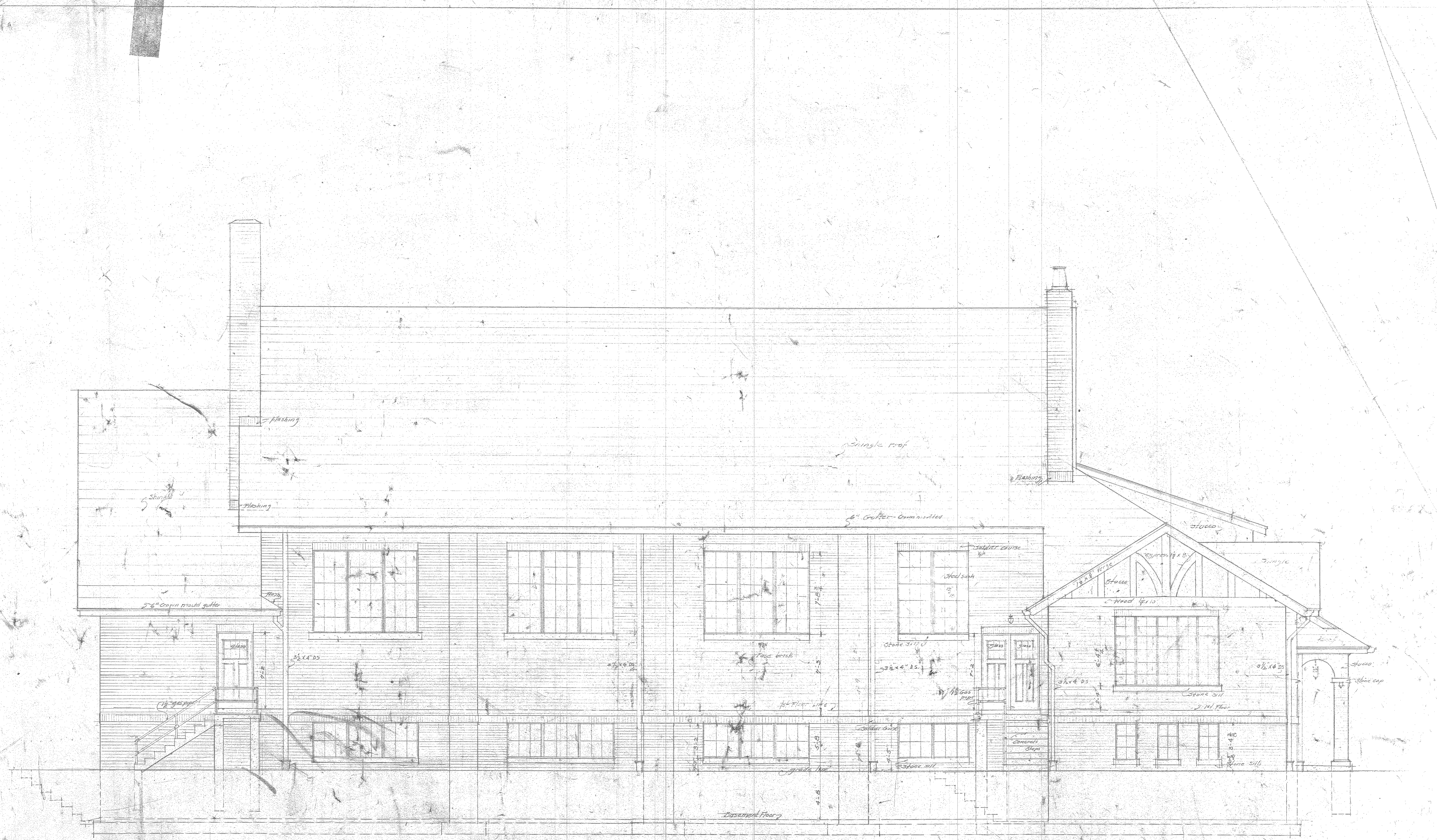
SOUTH SIDE ELEVATION Scale 1/4" = 1'-0"
